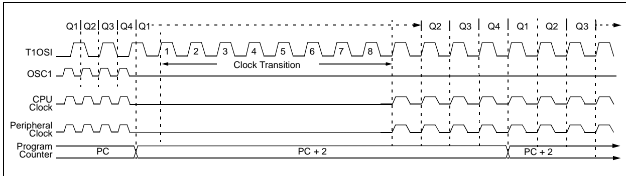
FIGURE 3-9: TIMING TRANSITION FOR ENTRY TO SEC_RUN MODE
