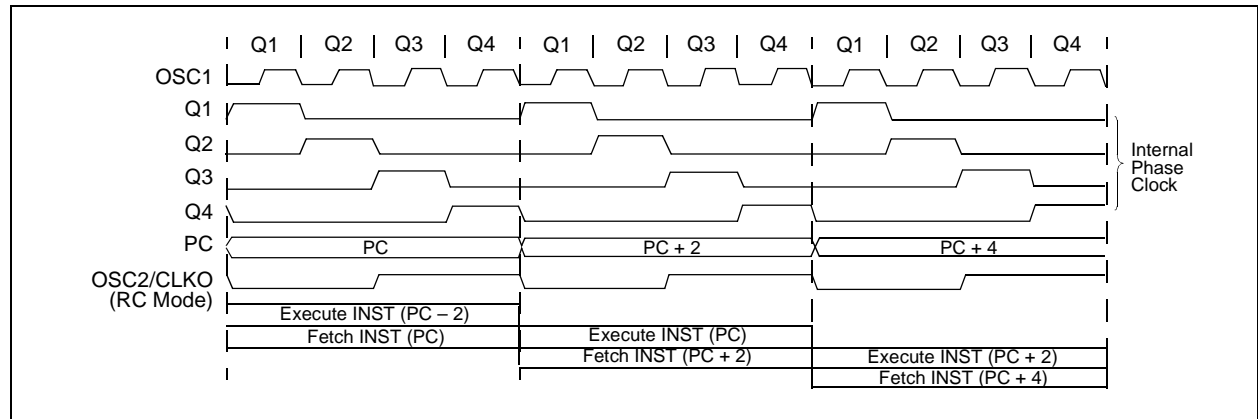
FIGURE 5-4: CLOCK/INSTRUCTION CYCLE
